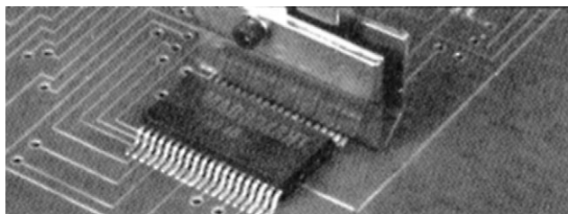
Reflow soldering multiple flat pack leads with multiple lead fold-up thermode. The fold-up design is electrically compatible with voltage sensitive components.
