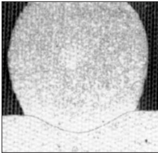
Solid State Bond
