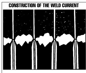
Exaggerated cross-section of two pieces of metal indicates formation of metallic bridges that result in high current density. Subsequent melting and the formation of new bridges allow the weld to be formed.
