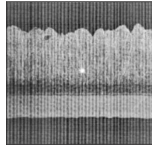
Reflow Braze Bond
