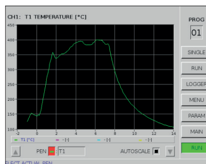
Temperature Graph
