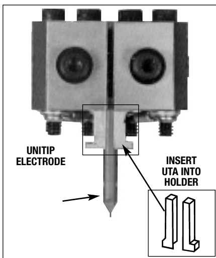
Model UTA UNITIP adapter. Use with 50F/UB, 50A/UB, 86F and 86A weld heads.
