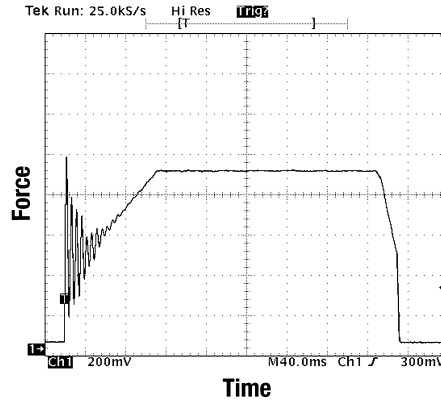
Force profile of TL-508B-2-EZ with EZ-AIR
