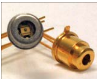
Projection welding small TO devices
