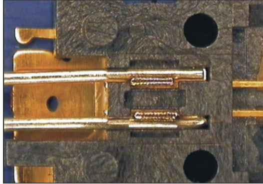
Figure 3 - 28 gauge gold coated copper wire to terminal LW2AG
