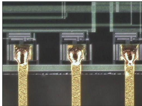
Figure 2 -LW2AG Semiconductor_connections
